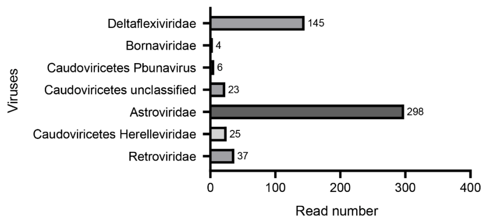
Supplementary Figure S1 Abundance of viruses in intestine of donkeys detected by mNGS
