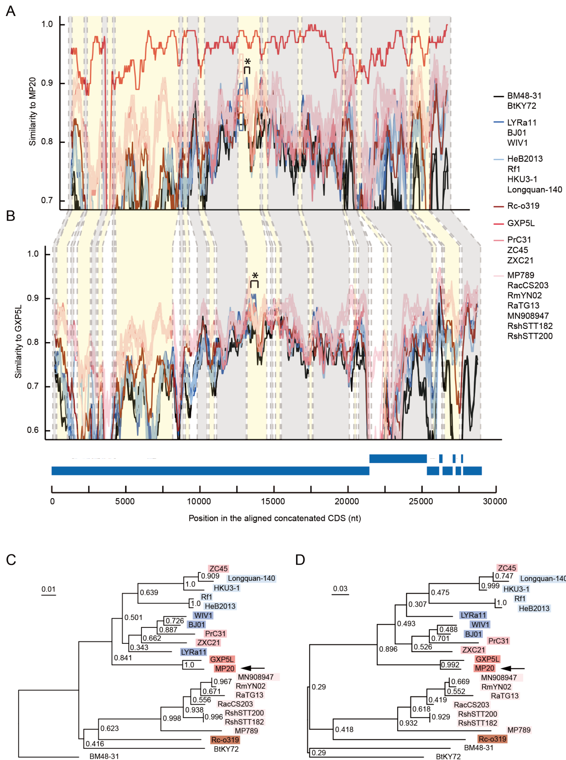
Figure 3 Recombination analysis of the pangolin-CoV-GXC sublineage
